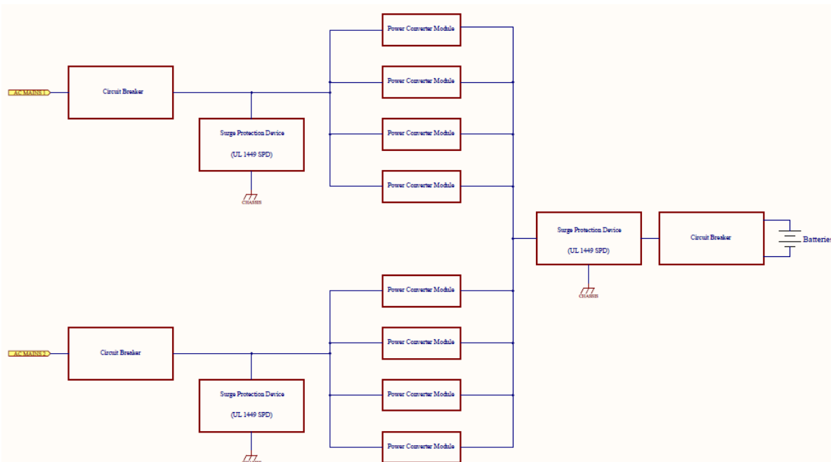
Figure 3. Simplified system-level diagram of modular switchmode battery charger system with dual AC feed
