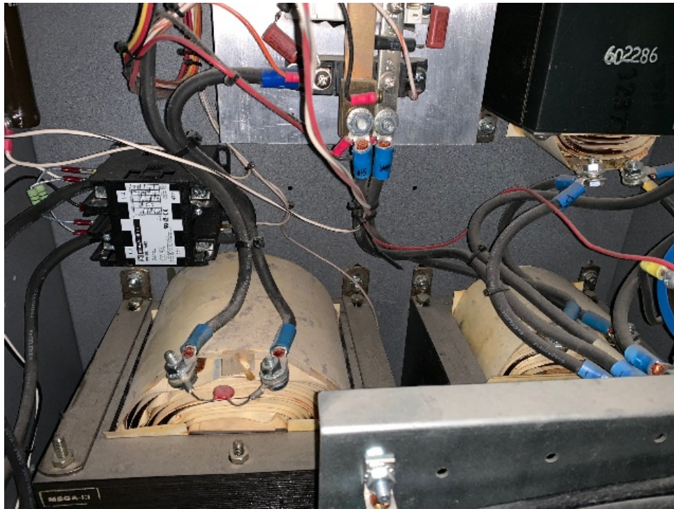
Figure 6. Minor dirt accumulation inside convection cooled SCR charger after 13 years
