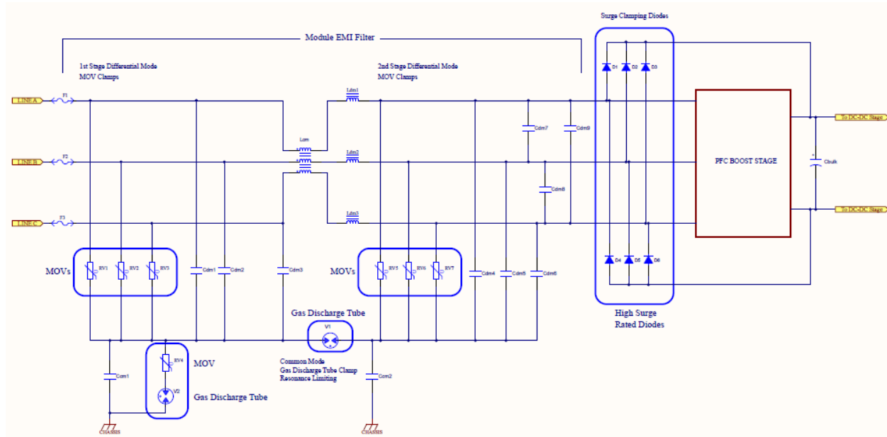
Figure 4. Simplified diagram of AC electrical transient protection in a 3-phase switchmode rectifier module
