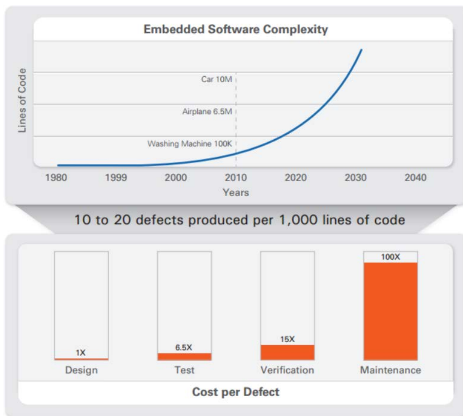
Figure 12 Growing Problem of Embedded Software Complexity 5
