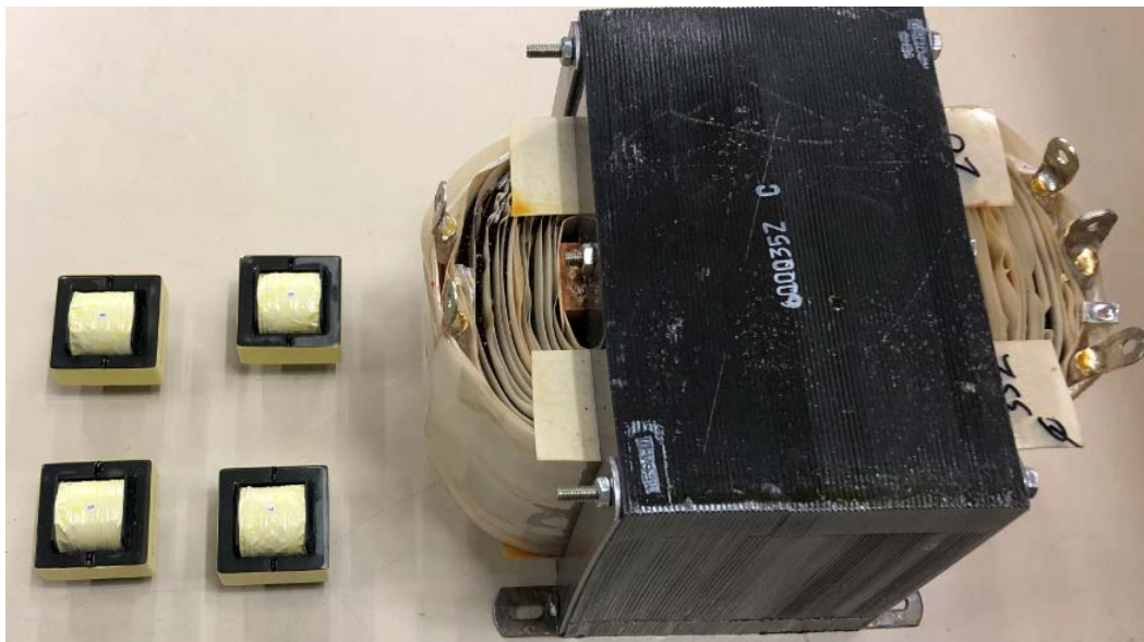
Figure 1. Switchmode & line frequency transformers for 7 kW charger; 2.7 lb. vs 127 lb.
