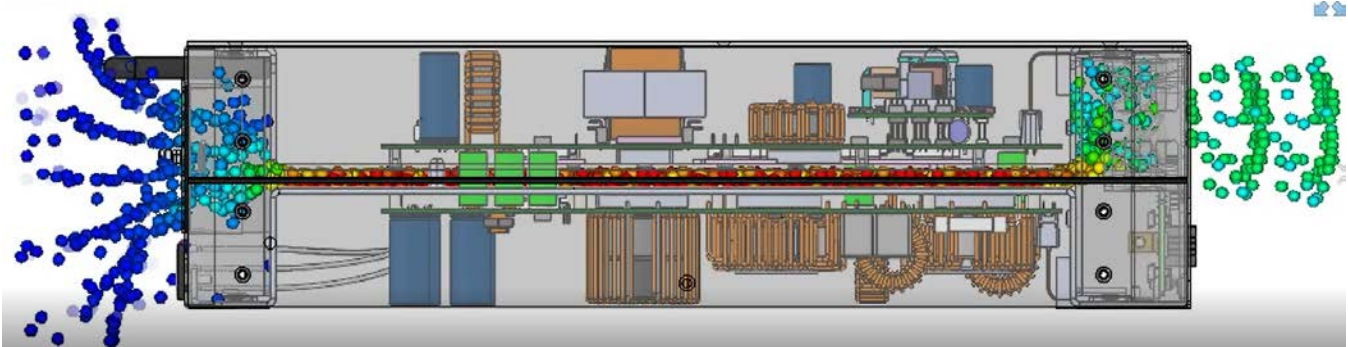
Figure 11. Side view of air flow isolated from electronic components. Color indicates relative velocity
