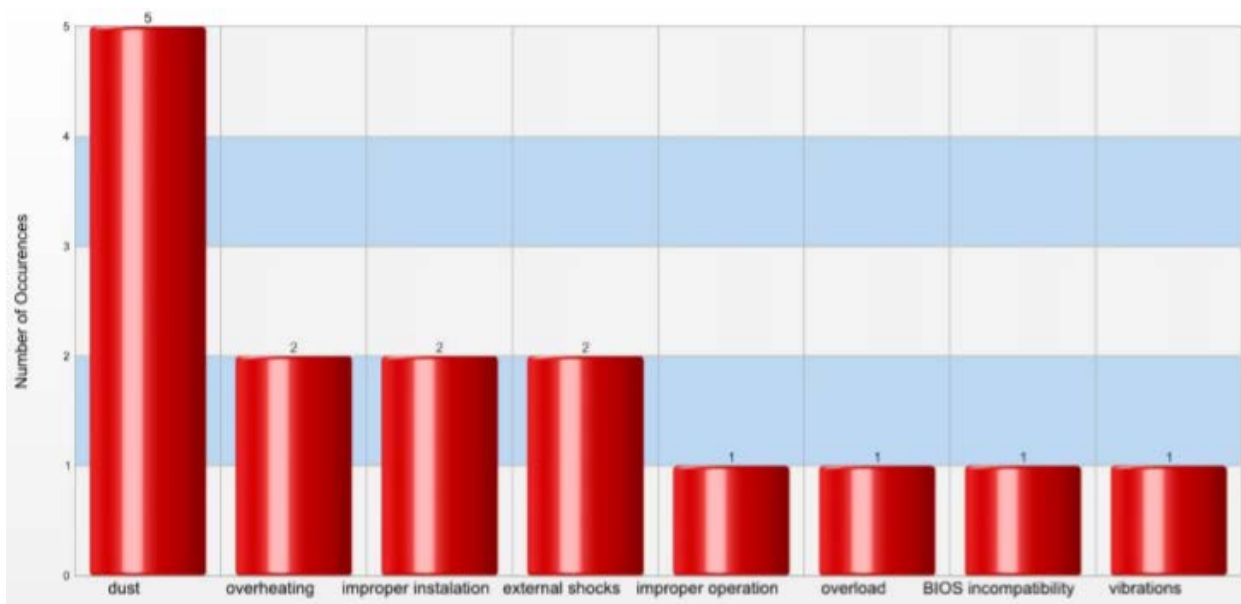
Figure 5. Leading causes of fan failure in computers 2
