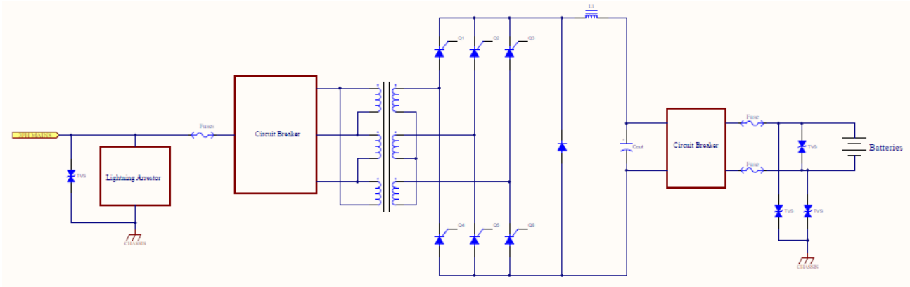
Figure 2. Simplified diagram of 3-phase input SCR type battery charger power train
